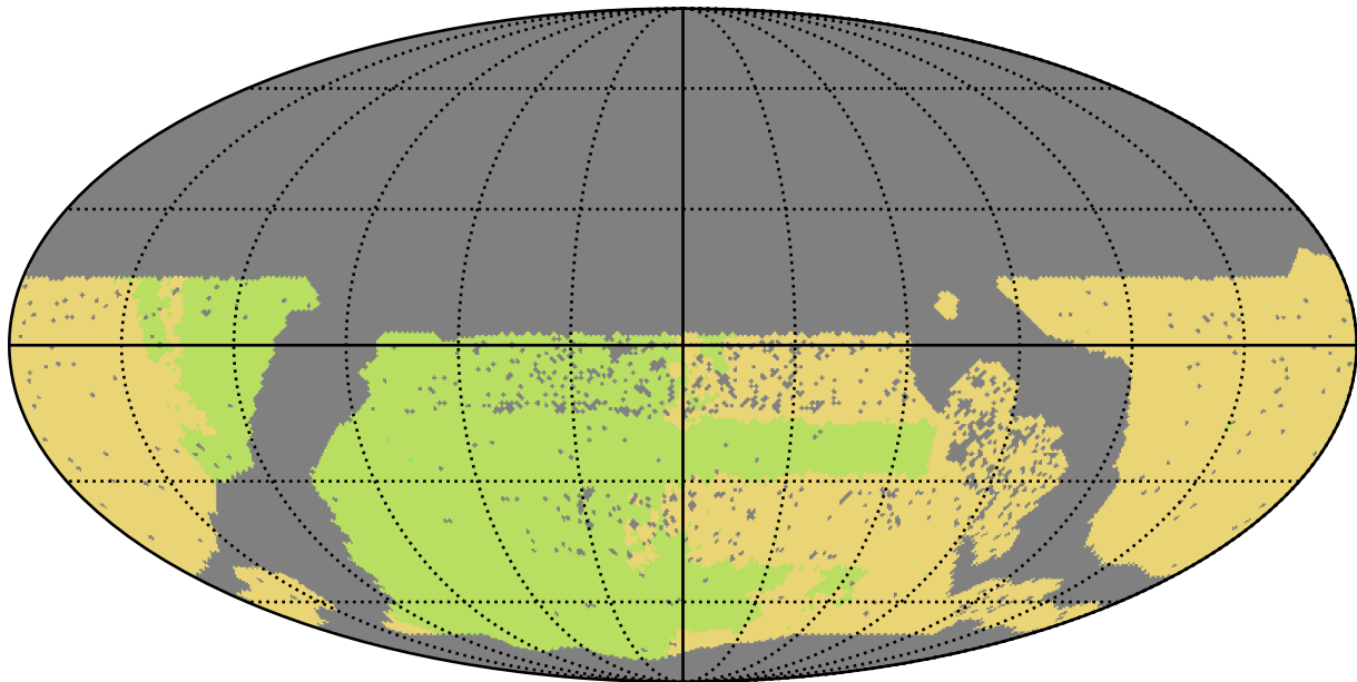
too_elab_r256_d3_griz_v3.4_10yrs WFD all bands: NSeasons
