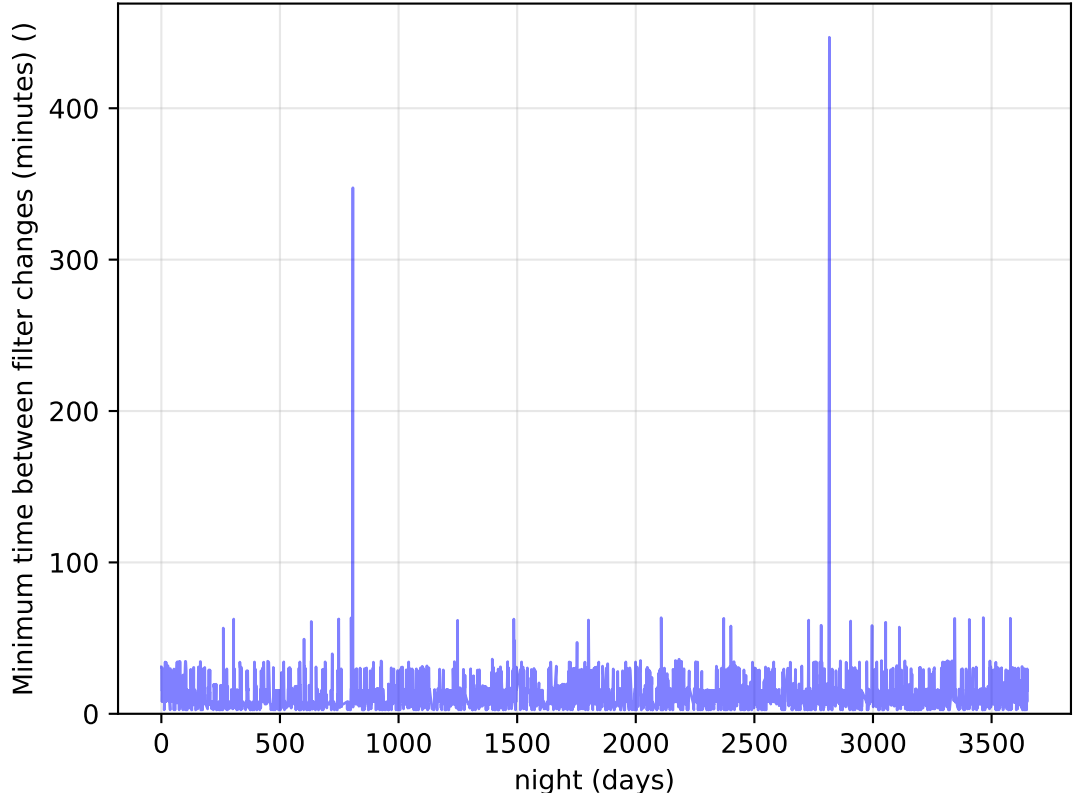
too_elab_r256_d3_griz_v3.4_10yrs Per Night: Minimum time between filter changes (minutes)
