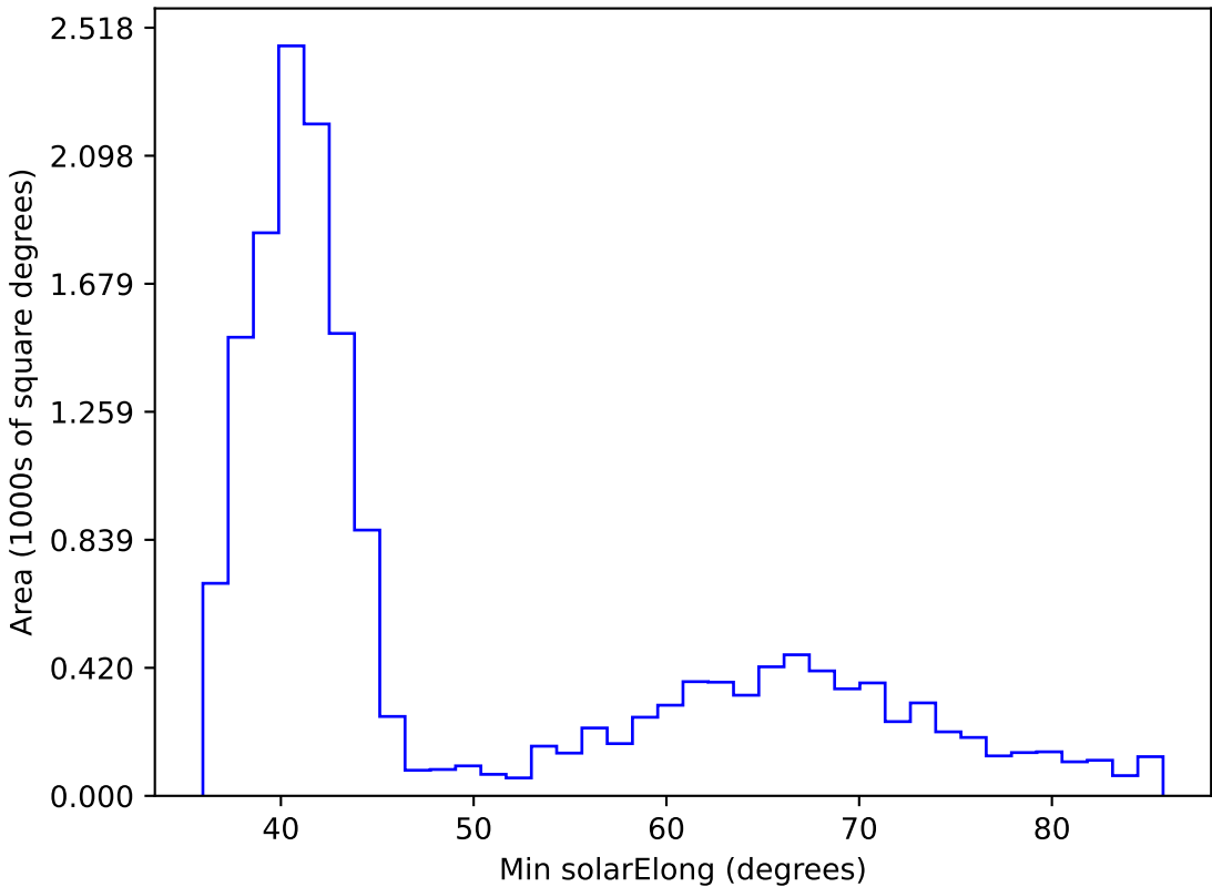
too_elab_r256_d3_griz_v3.4_10yrs WFD z band: Min solarElong
