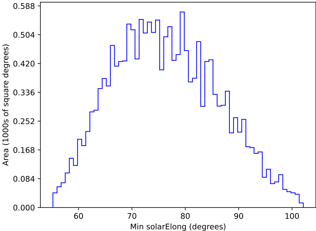
too_elab_r256_d3_griz_v3.4_10yrs WFD u band: Min solarElong
