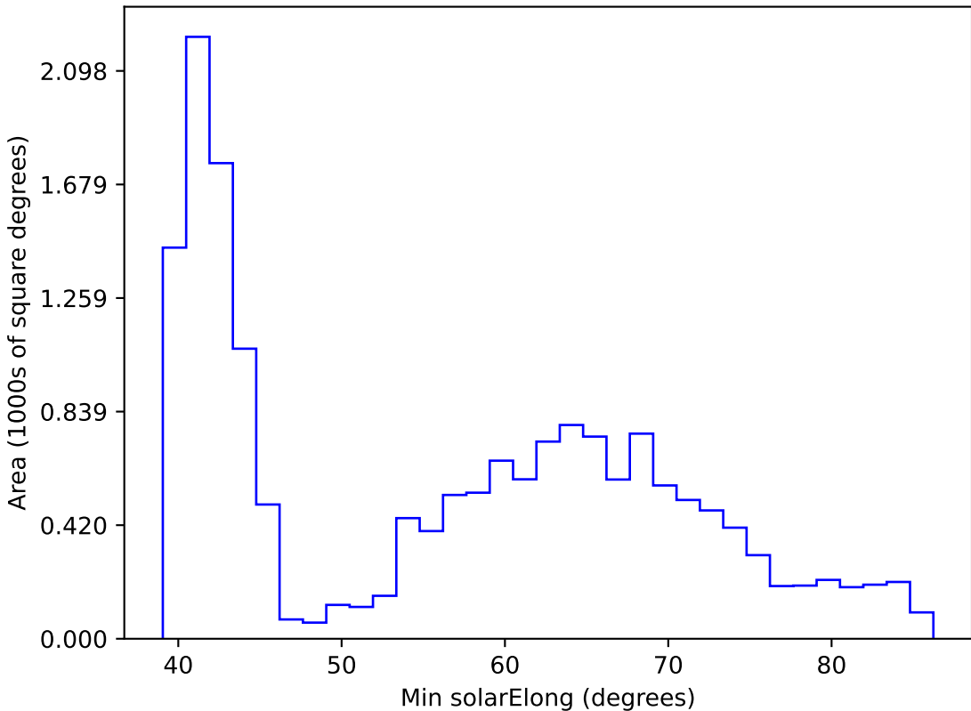
too_elab_r256_d3_griz_v3.4_10yrs WFD r band: Min solarElong
