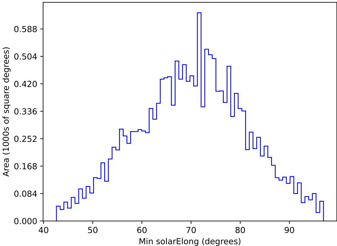
too_elab_r256_d3_griz_v3.4_10yrs WFD g band: Min solarElong
