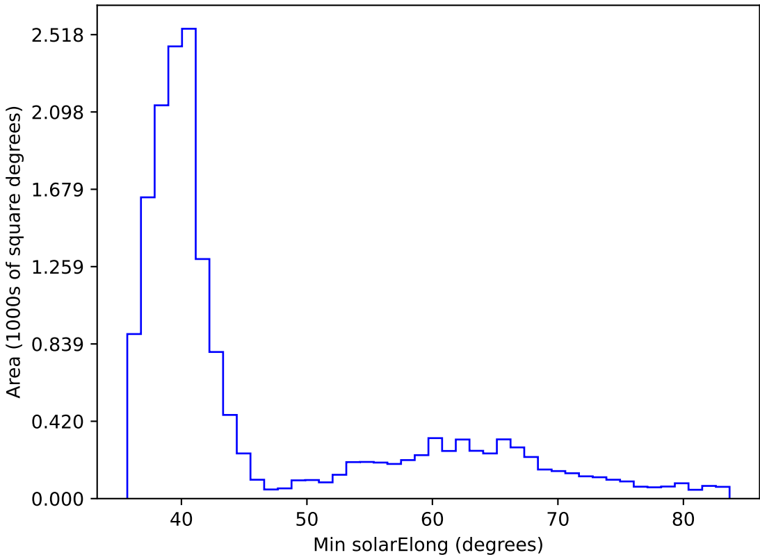
too_elab_r256_d3_griz_v3.4_10yrs WFD all bands: Min solarElong
