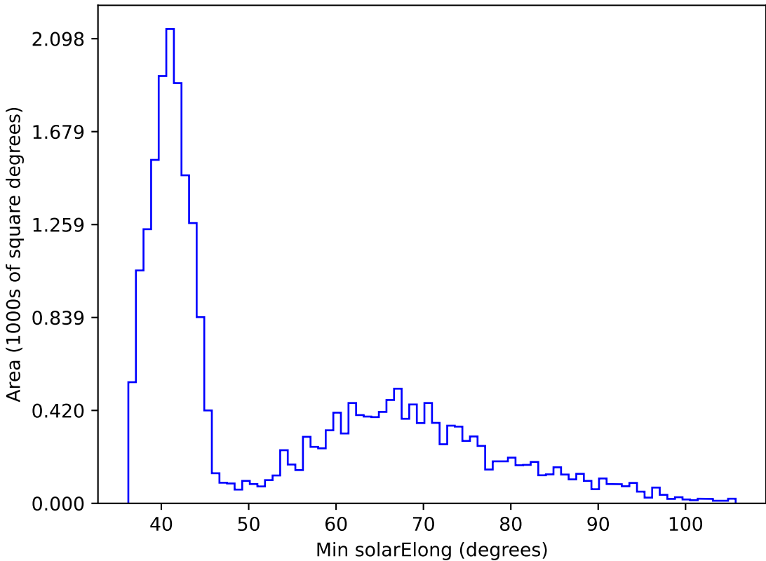
too_elab_r256_d3_griz_v3.4_10yrs All sky z band: Min solarElong
