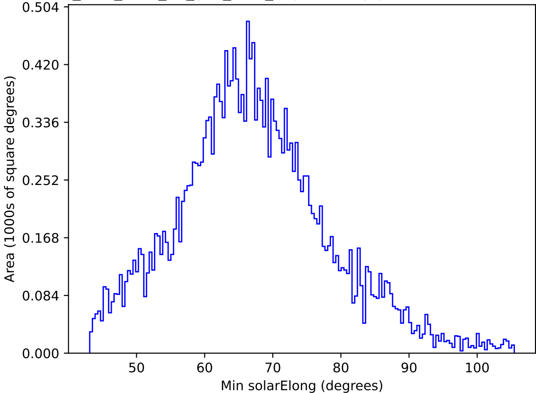
too_elab_r256_d3_griz_v3.4_10yrs All sky y band: Min solarElong
