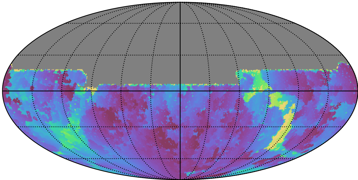
too_elab_r256_d3_griz_v3.4_10yrs All sky u band: Min solarElong
