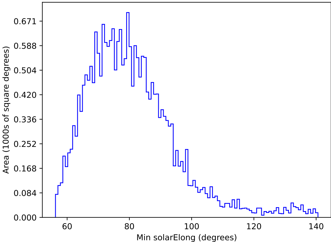
too_elab_r256_d3_griz_v3.4_10yrs All sky u band: Min solarElong
