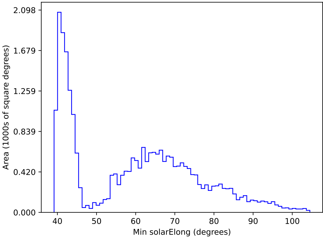
too_elab_r256_d3_griz_v3.4_10yrs All sky r band: Min solarElong
