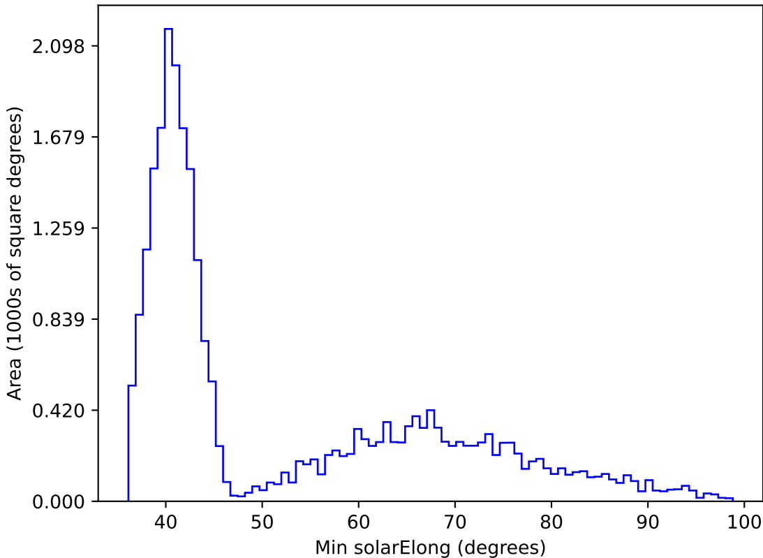
too_elab_r256_d3_griz_v3.4_10yrs All sky i band: Min solarElong
