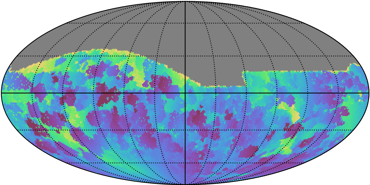
too_elab_r256_d3_griz_v3.4_10yrs All sky g band: Min solarElong
