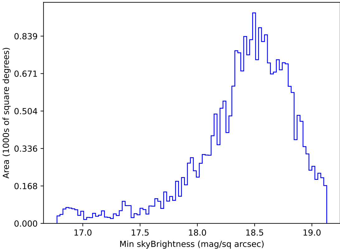
too_elab_r256_d3_griz_v3.4_10yrs Yr 1 z band: Min skyBrightness
