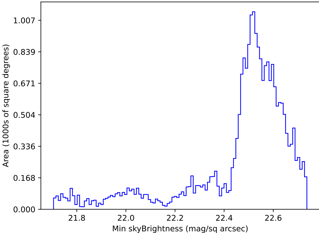
too_elab_r256_d3_griz_v3.4_10yrs Yr 1 u band: Min skyBrightness
