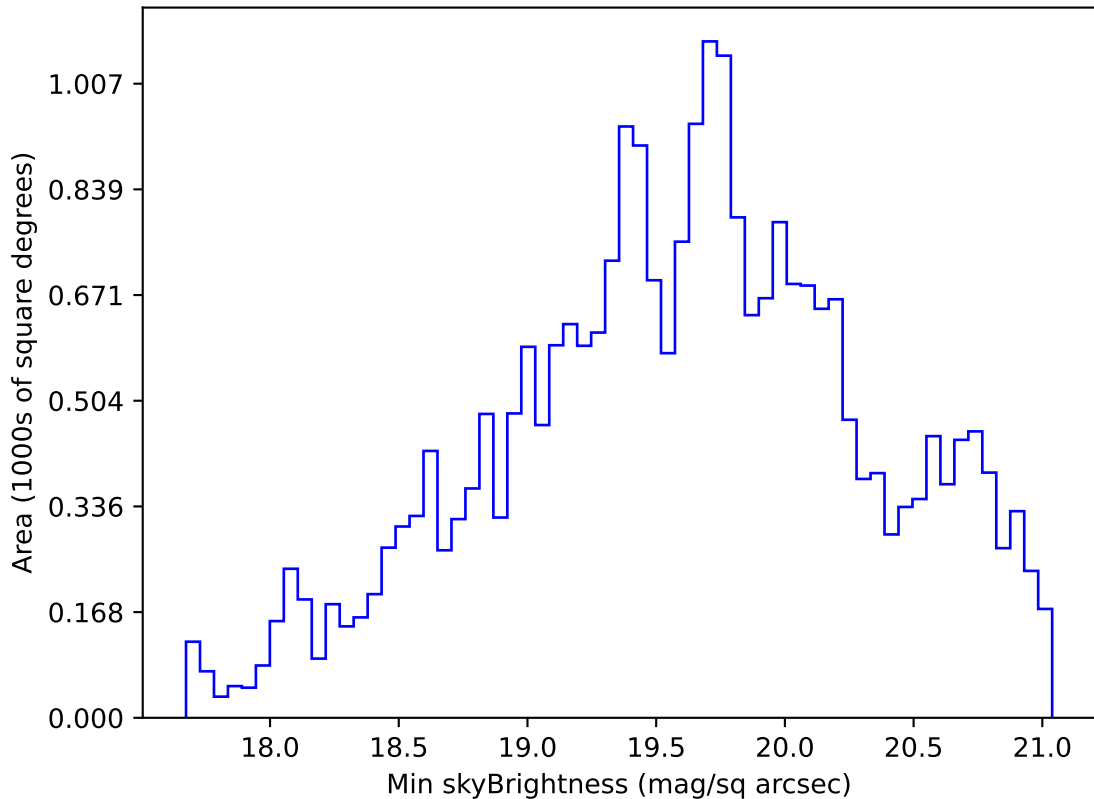
too_elab_r256_d3_griz_v3.4_10yrs Yr 1 r band: Min skyBrightness
