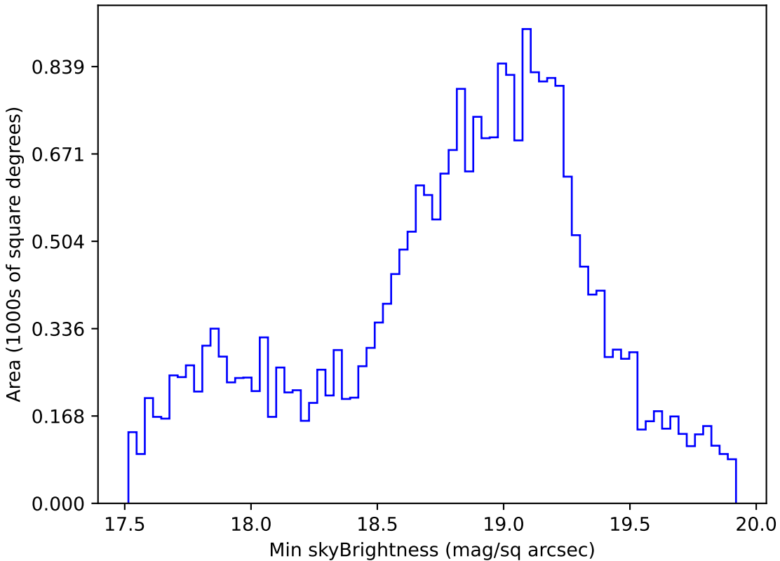
too_elab_r256_d3_griz_v3.4_10yrs Yr 1 i band: Min skyBrightness
