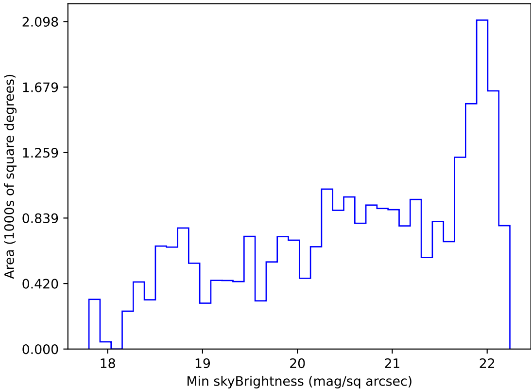
too_elab_r256_d3_griz_v3.4_10yrs Yr 1 g band: Min skyBrightness
