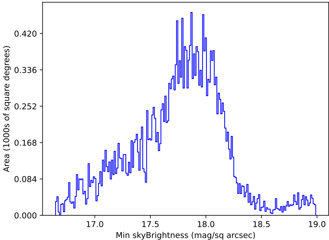
too_elab_r256_d3_griz_v3.4_10yrs Yr 1 all bands: Min skyBrightness
