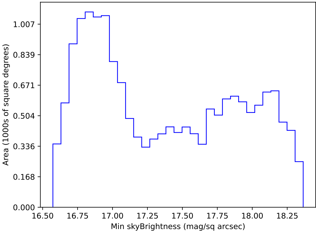
too_elab_r256_d3_griz_v3.4_10yrs WFD z band: Min skyBrightness
