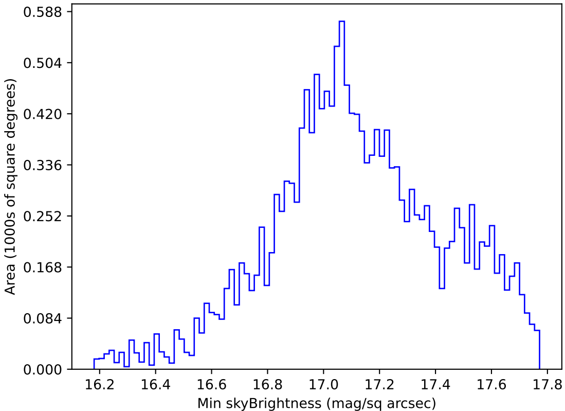
too_elab_r256_d3_griz_v3.4_10yrs WFD y band: Min skyBrightness
