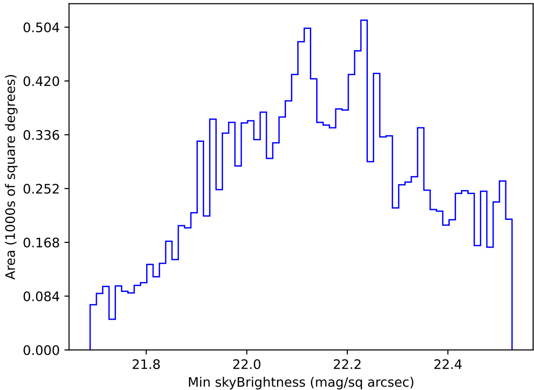
too_elab_r256_d3_griz_v3.4_10yrs WFD u band: Min skyBrightness
