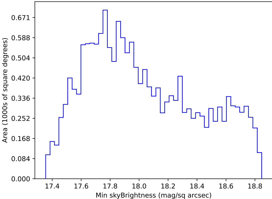
too_elab_r256_d3_griz_v3.4_10yrs WFD i band: Min skyBrightness
