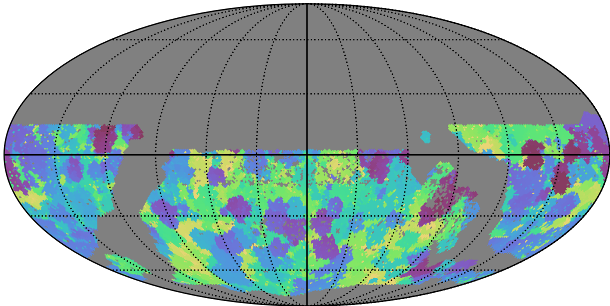
too_elab_r256_d3_griz_v3.4_10yrs WFD g band: Min skyBrightness
