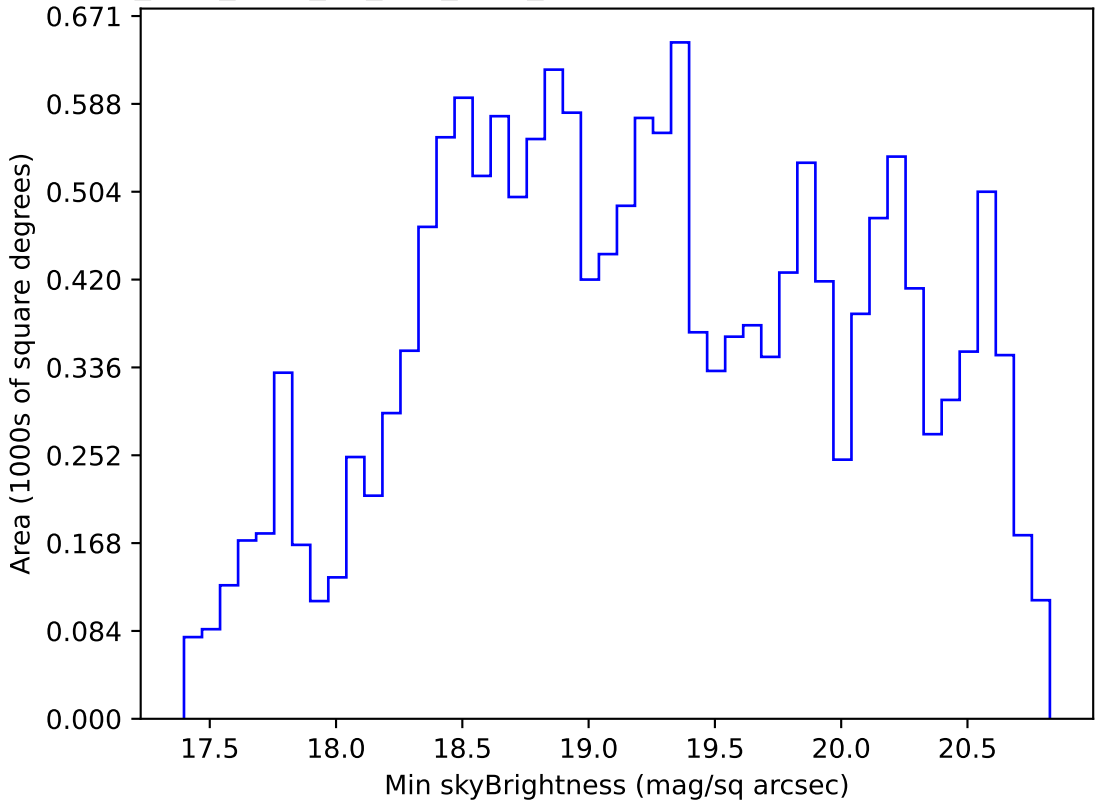
too_elab_r256_d3_griz_v3.4_10yrs WFD g band: Min skyBrightness
