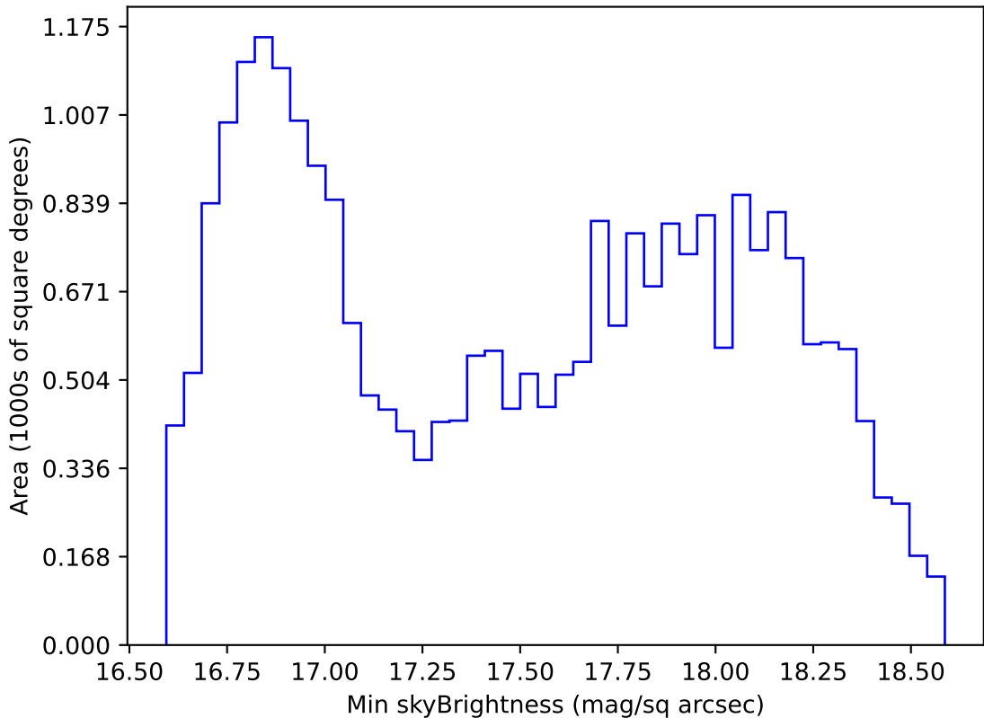
too_elab_r256_d3_griz_v3.4_10yrs All sky z band: Min skyBrightness
