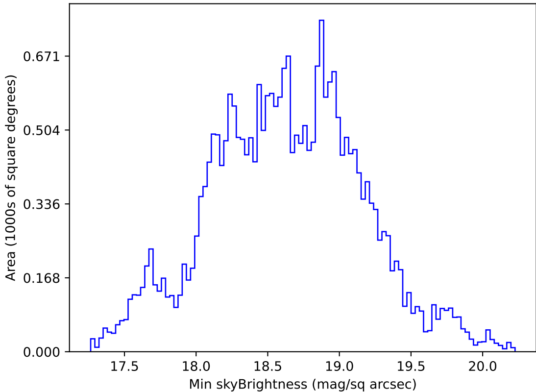
too_elab_r256_d3_griz_v3.4_10yrs All sky r band: Min skyBrightness
