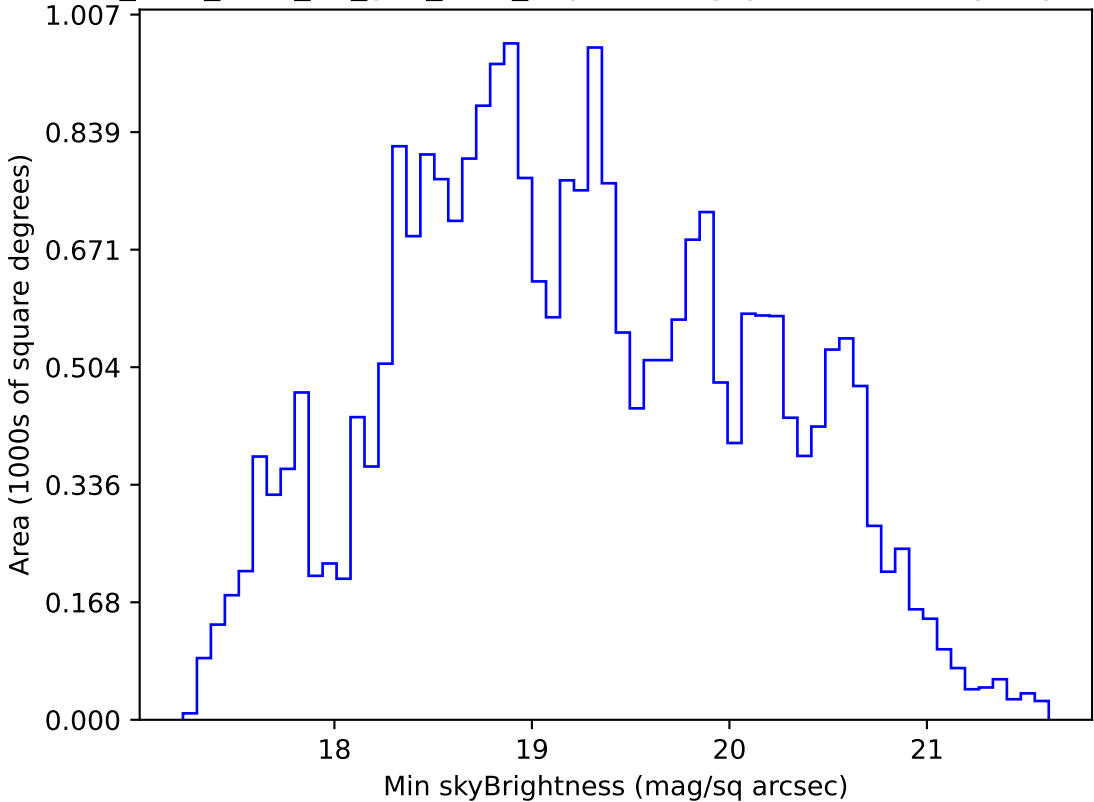
too_elab_r256_d3_griz_v3.4_10yrs All sky g band: Min skyBrightness
