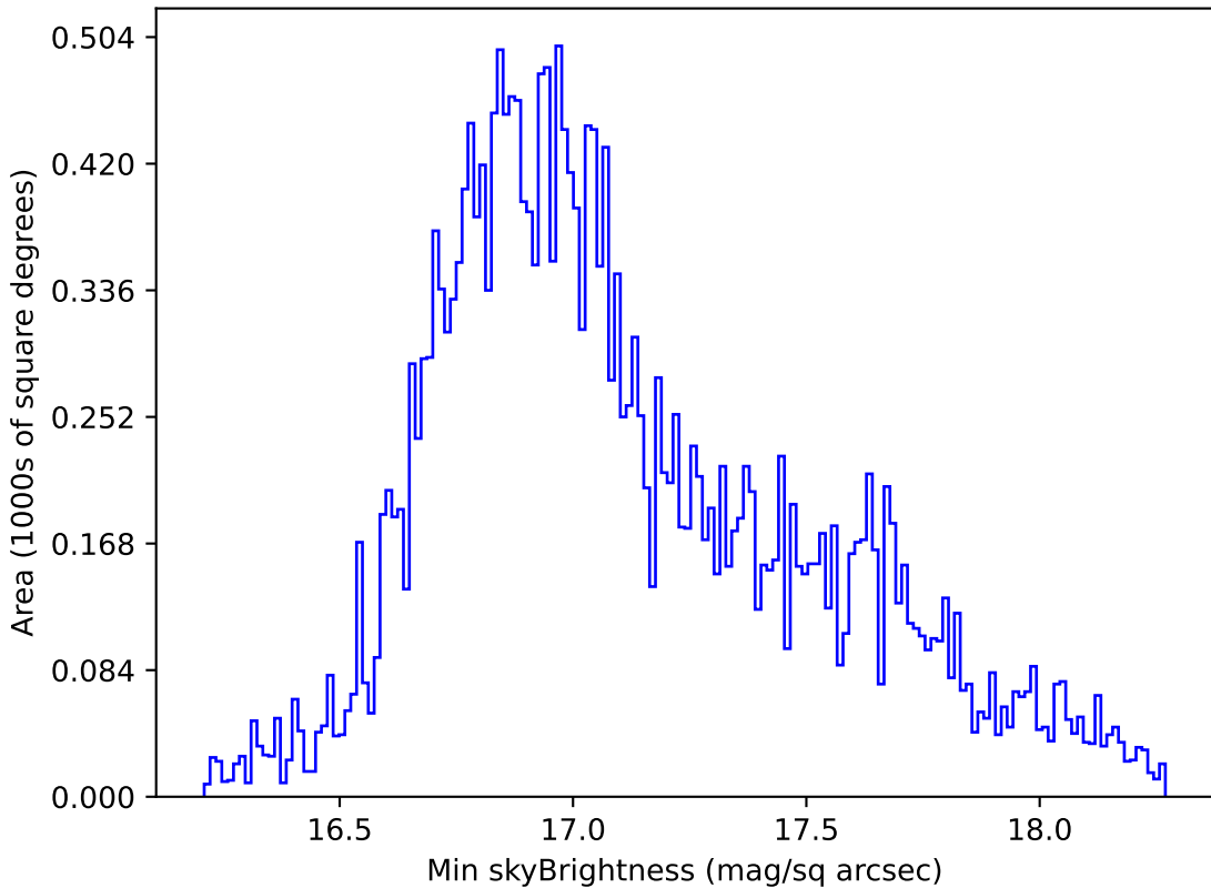
too_elab_r256_d3_griz_v3.4_10yrs All sky all bands: Min skyBrightness
