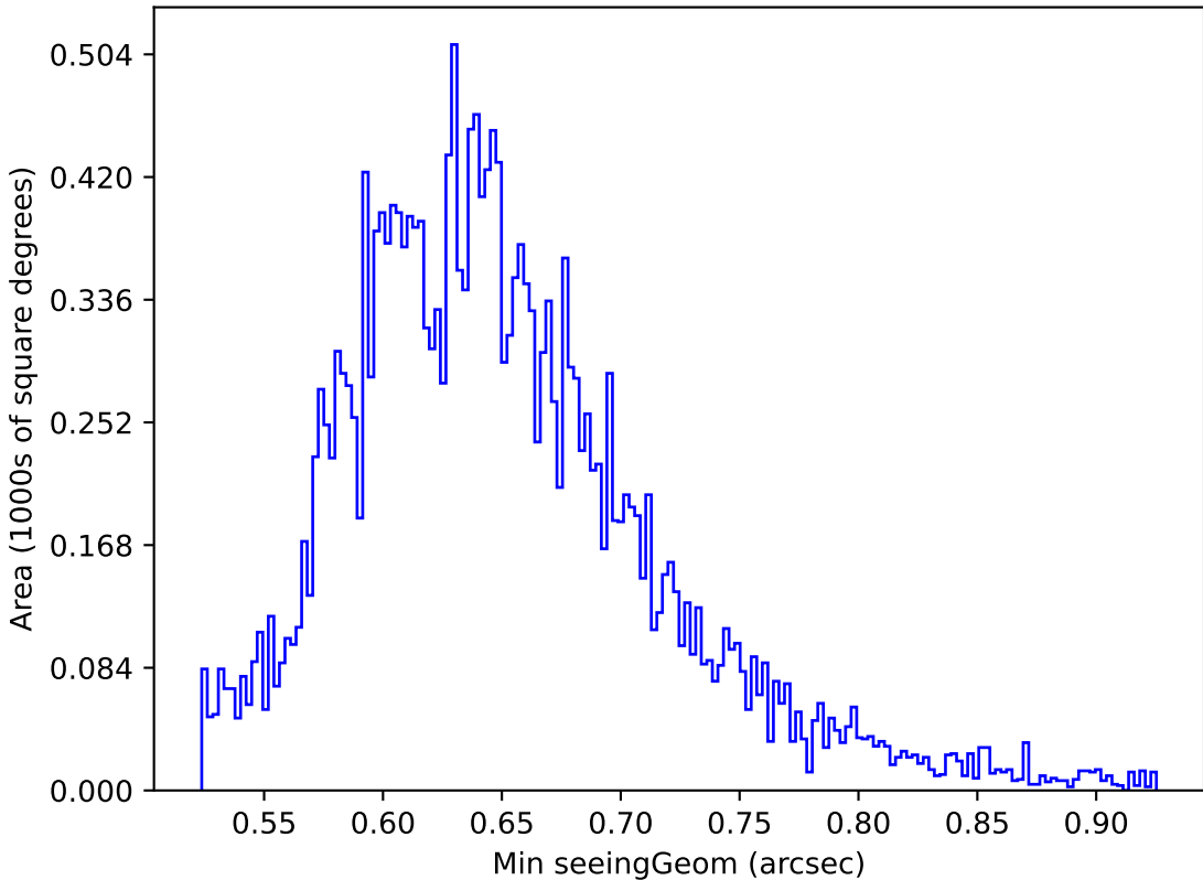
too_elab_r256_d3_griz_v3.4_10yrs Yr 1 y band: Min seeingGeom
