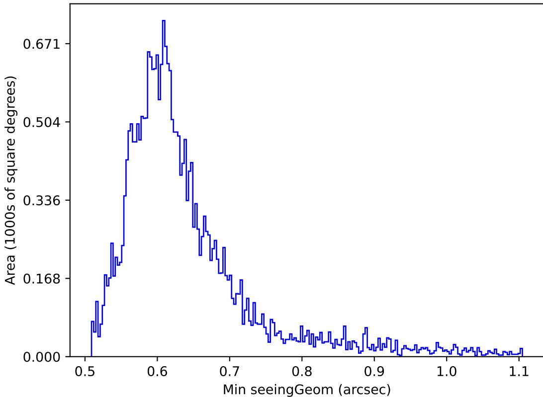
too_elab_r256_d3_griz_v3.4_10yrs Yr 1 r band: Min seeingGeom
