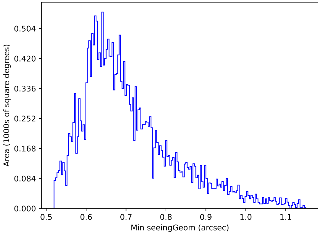
too_elab_r256_d3_griz_v3.4_10yrs Yr 1 g band: Min seeingGeom
