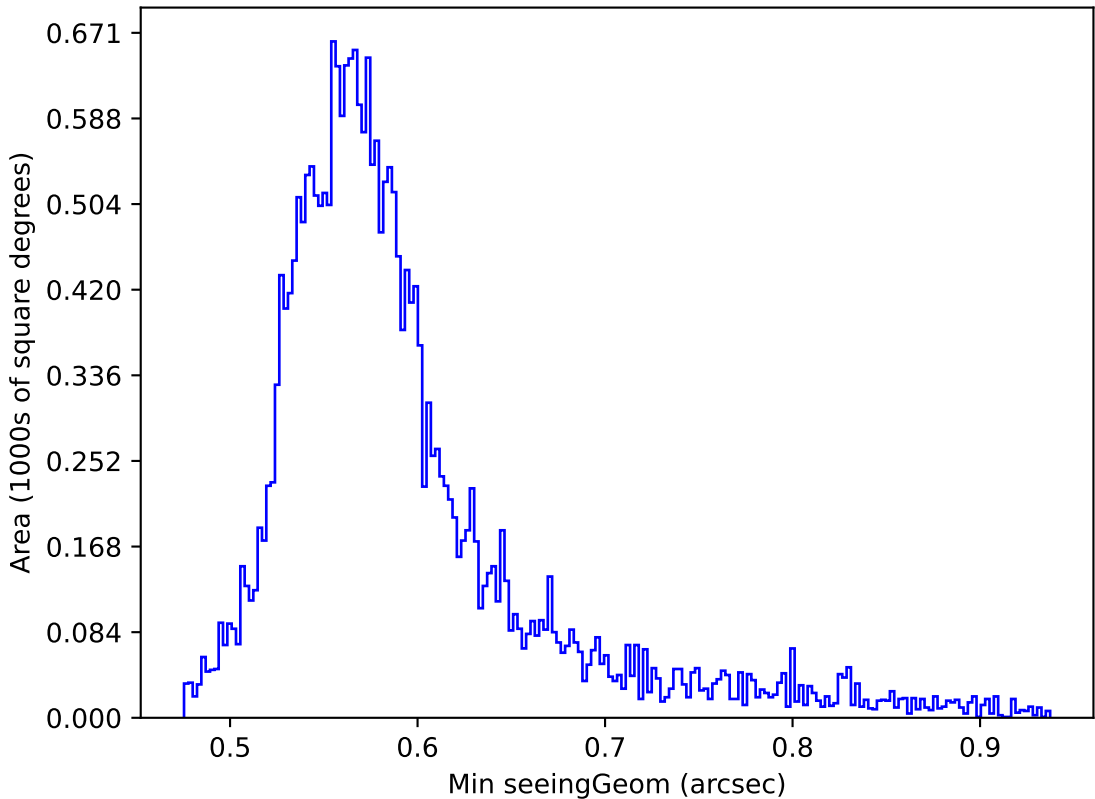
too_elab_r256_d3_griz_v3.4_10yrs Yr 1 all bands: Min seeingGeom
