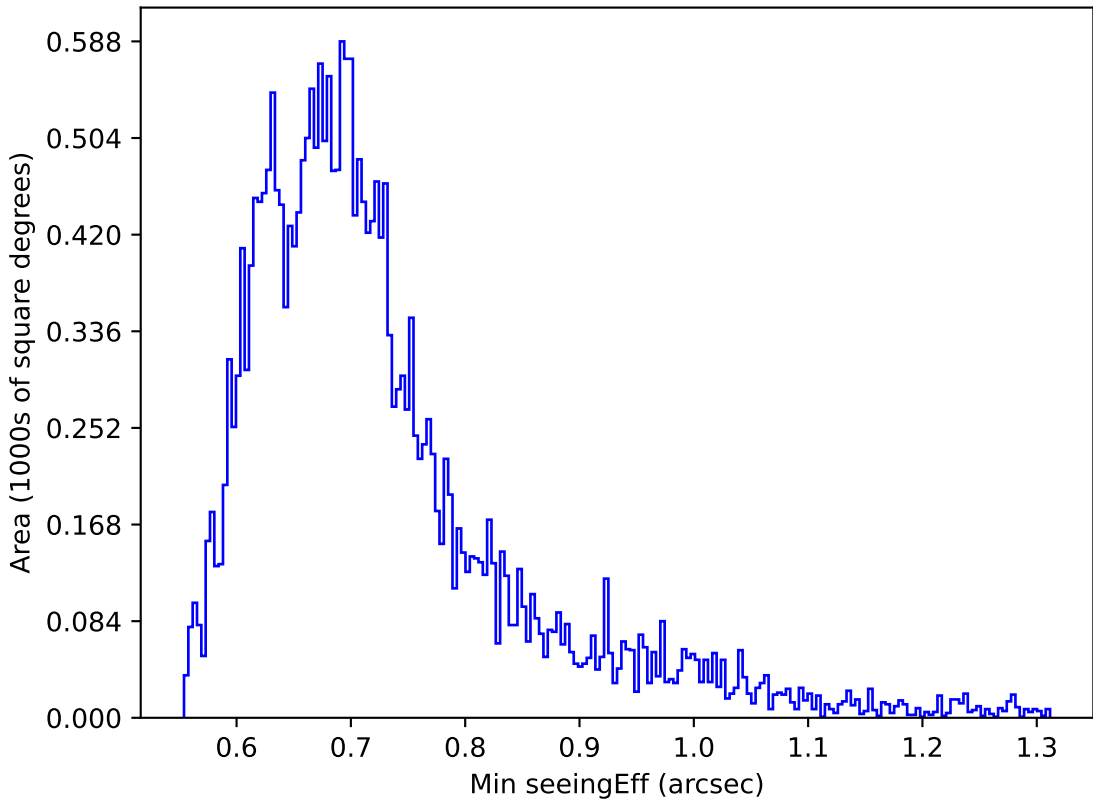
too_elab_r256_d3_griz_v3.4_10yrs Yr 1 z band: Min seeingEff
