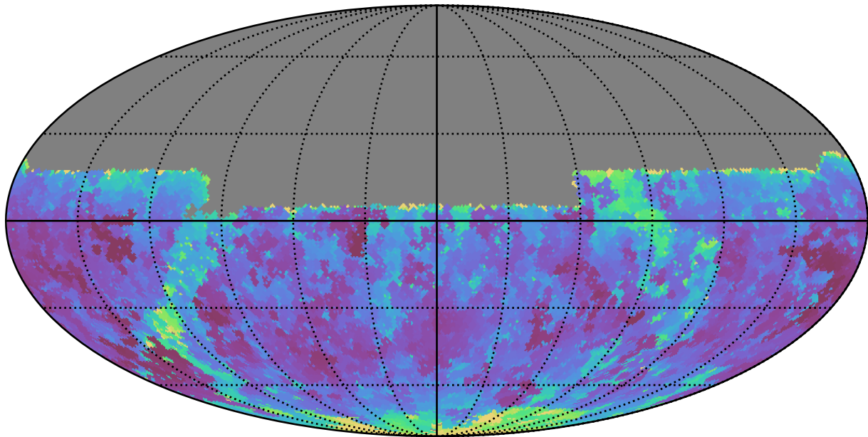
too_elab_r256_d3_griz_v3.4_10yrs Yr 1 y band: Min seeingEff
