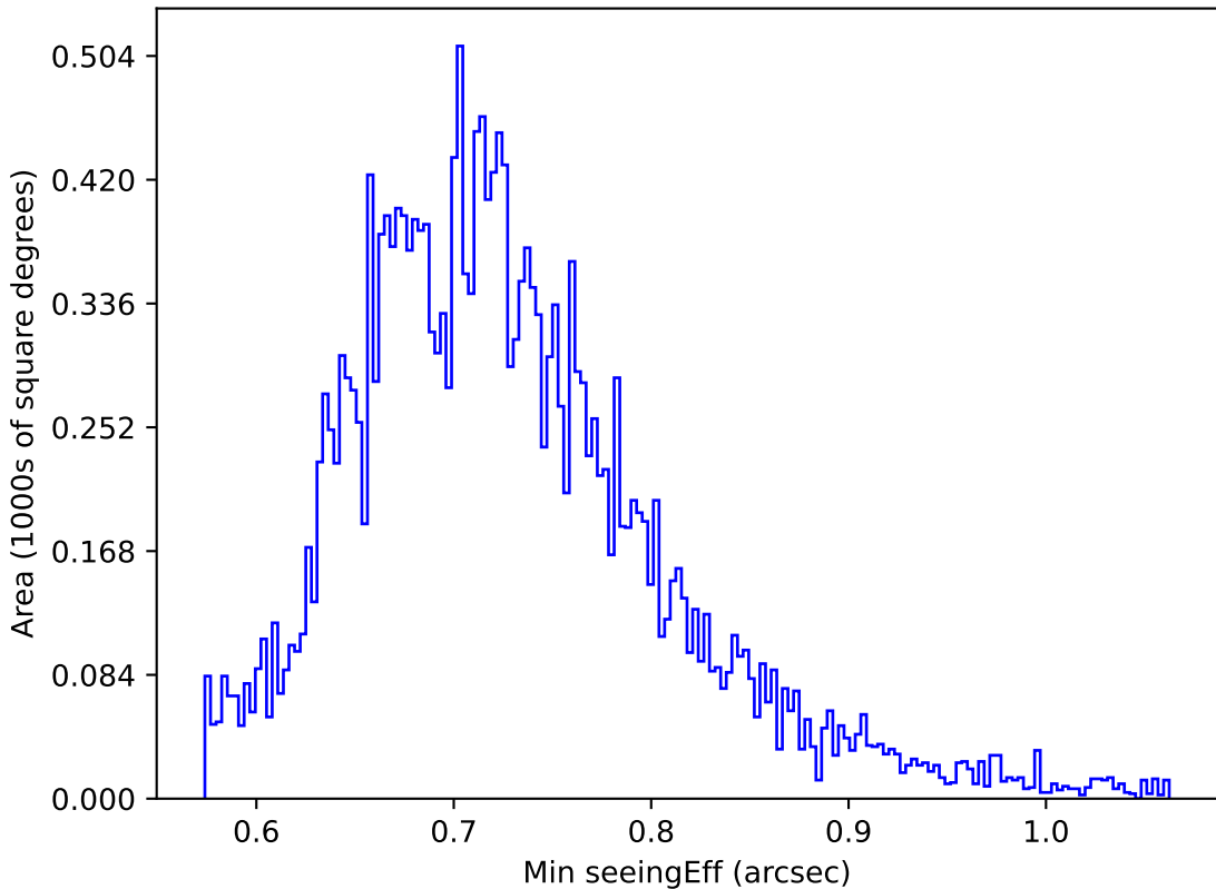
too_elab_r256_d3_griz_v3.4_10yrs Yr 1 y band: Min seeingEff
