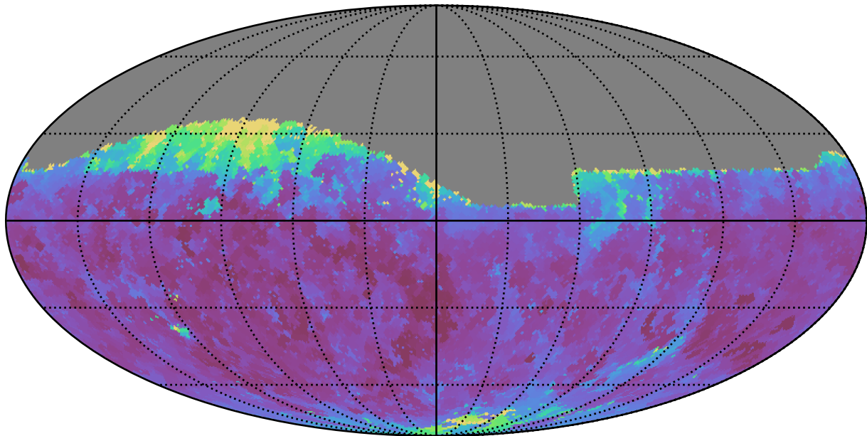
too_elab_r256_d3_griz_v3.4_10yrs Yr 1 r band: Min seeingEff
