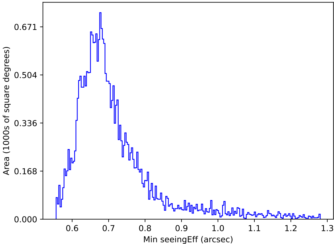
too_elab_r256_d3_griz_v3.4_10yrs Yr 1 r band: Min seeingEff
