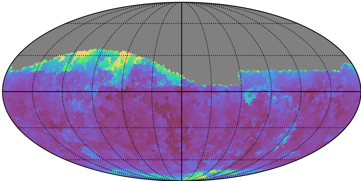
too_elab_r256_d3_griz_v3.4_10yrs Yr 1 i band: Min seeingEff
