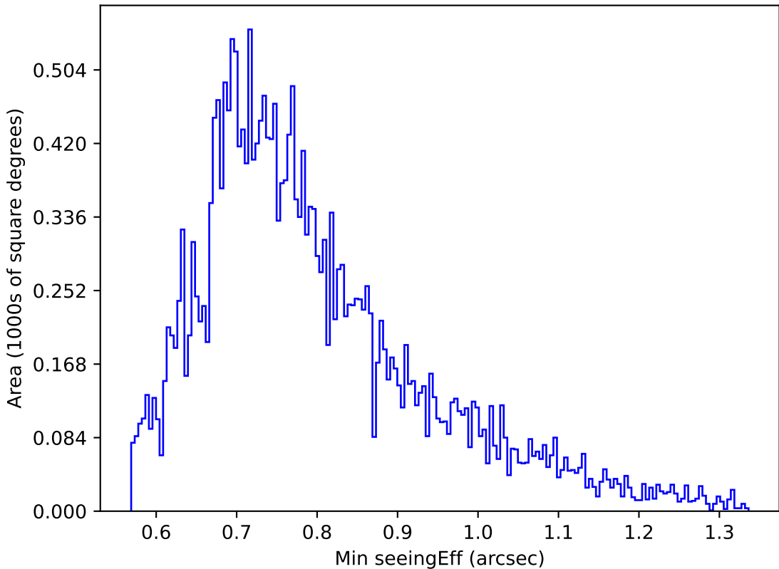
too_elab_r256_d3_griz_v3.4_10yrs Yr 1 g band: Min seeingEff
