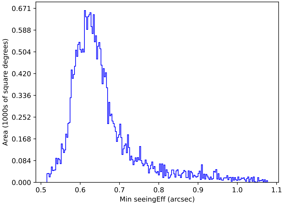
too_elab_r256_d3_griz_v3.4_10yrs Yr 1 all bands: Min seeingEff
