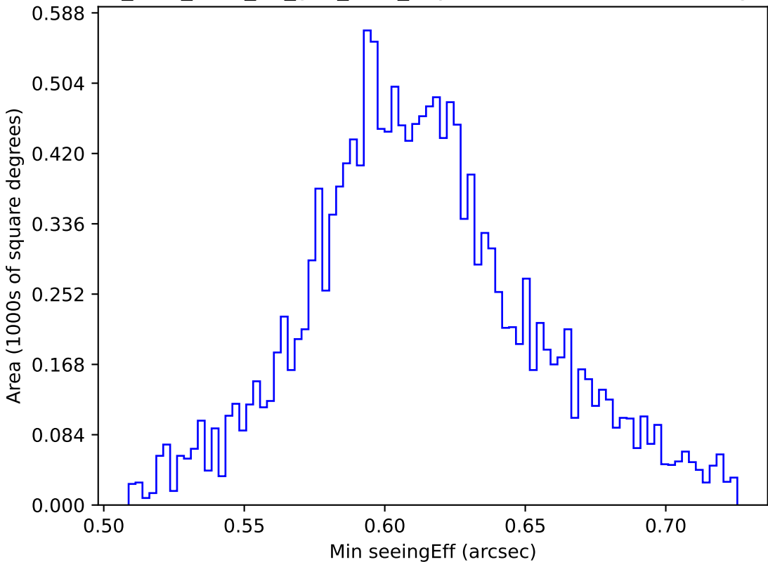
too_elab_r256_d3_griz_v3.4_10yrs WFD z band: Min seeingEff
