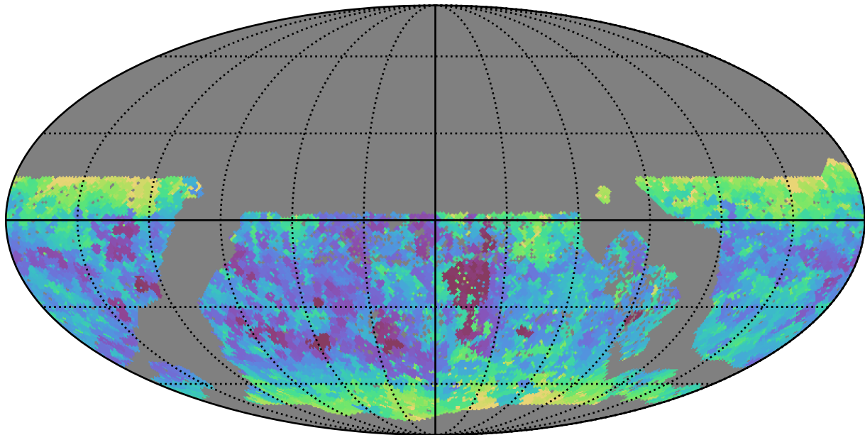
too_elab_r256_d3_griz_v3.4_10yrs WFD y band: Min seeingEff
