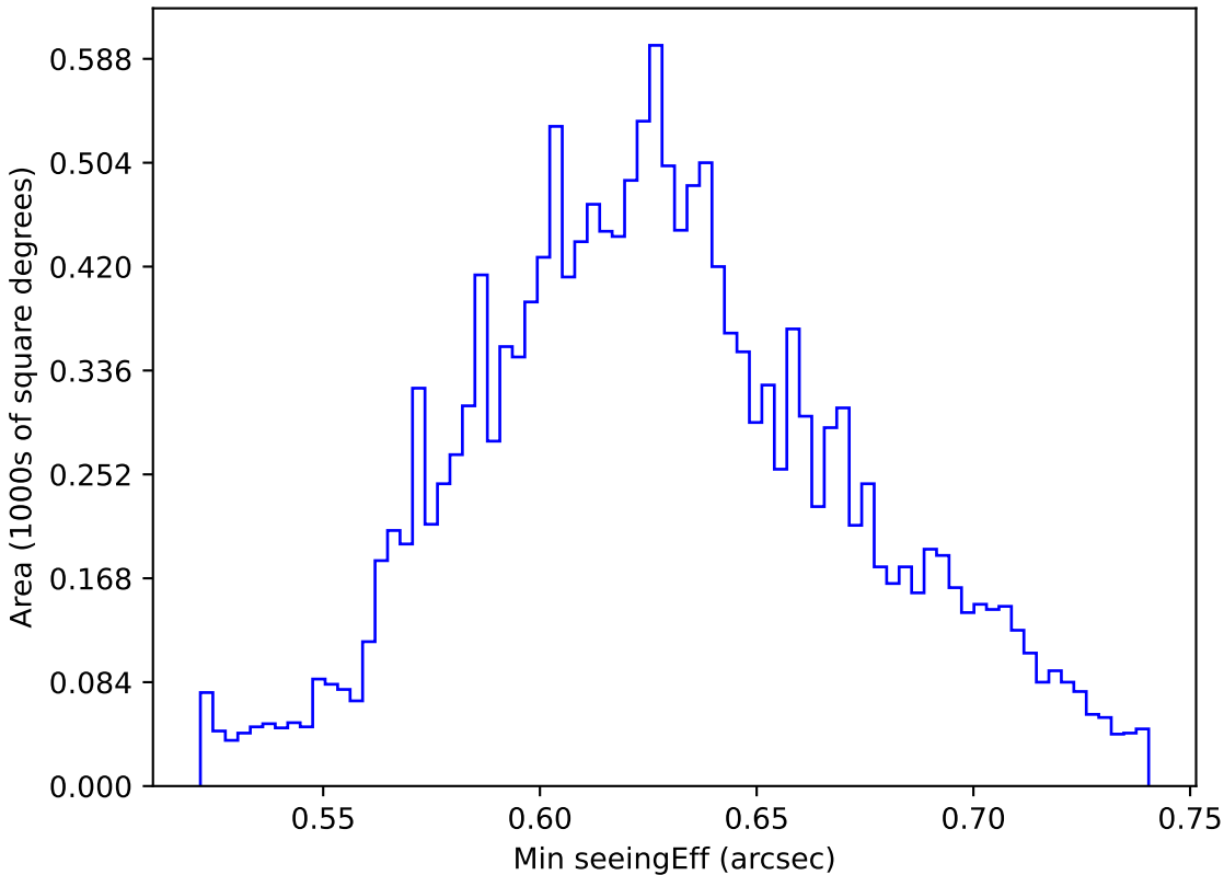
too_elab_r256_d3_griz_v3.4_10yrs WFD y band: Min seeingEff
