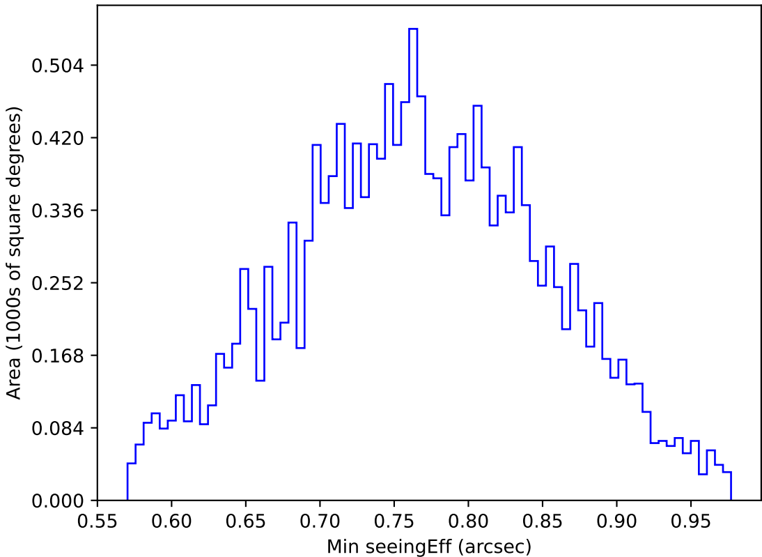
too_elab_r256_d3_griz_v3.4_10yrs WFD u band: Min seeingEff
