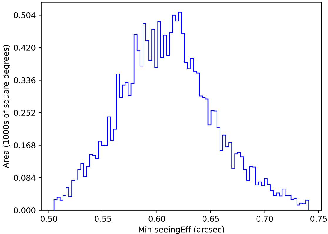
too_elab_r256_d3_griz_v3.4_10yrs WFD r band: Min seeingEff
