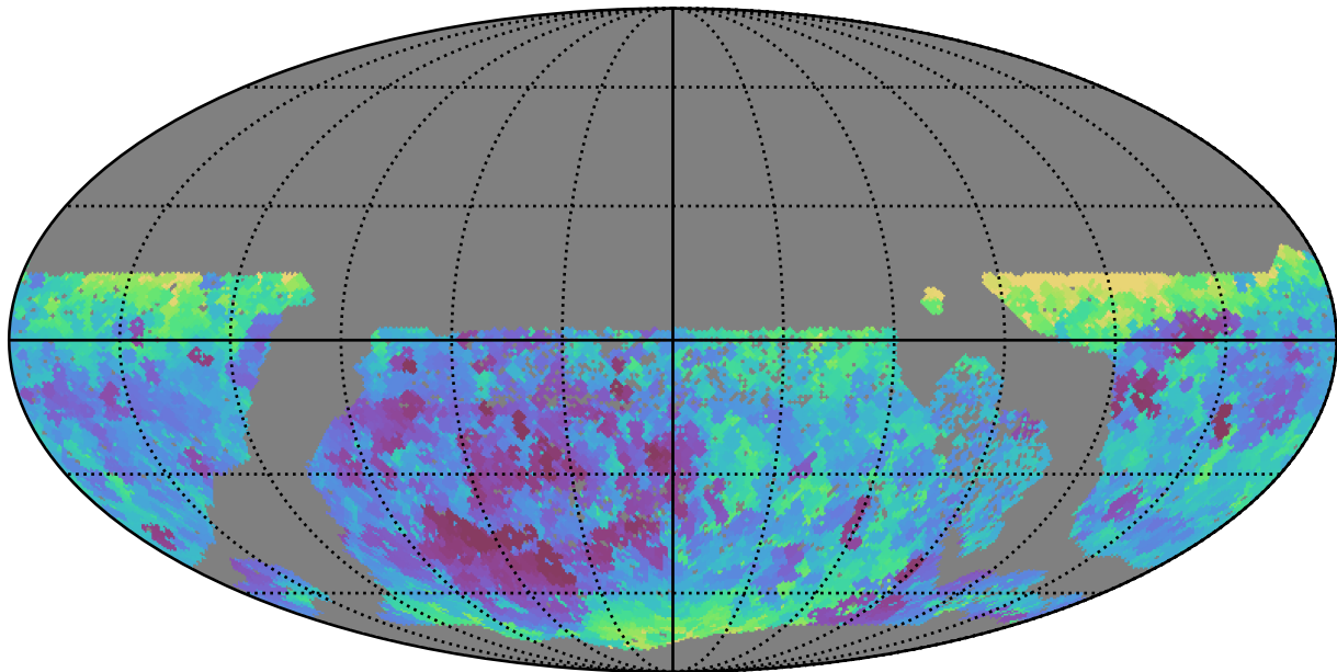
too_elab_r256_d3_griz_v3.4_10yrs WFD i band: Min seeingEff
