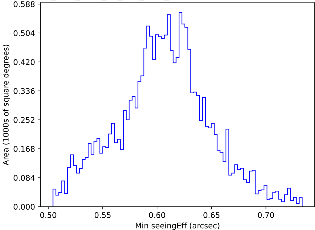
too_elab_r256_d3_griz_v3.4_10yrs WFD i band: Min seeingEff
