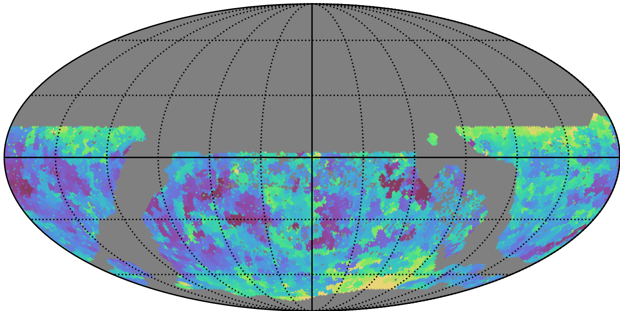
too_elab_r256_d3_griz_v3.4_10yrs WFD g band: Min seeingEff
